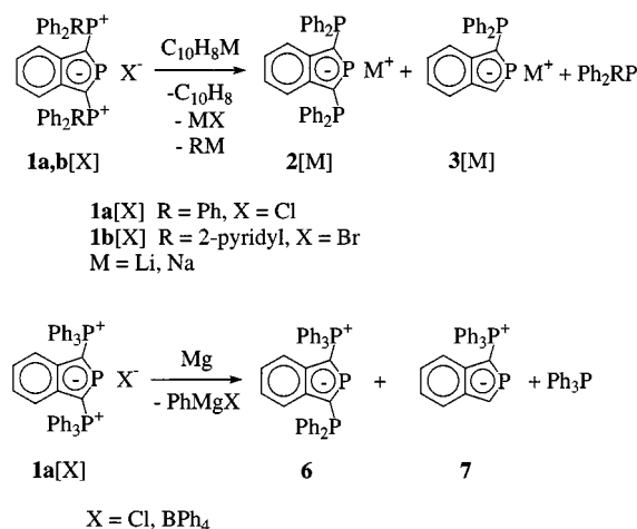
Scheme 1. \text{X} = \text{Cl, Br, BPh}_4 ; \text{M} = \text{Li, Na} ; \text{R} = \text{Ph} ( 1a ), 2-pyridyl ( 1b )
