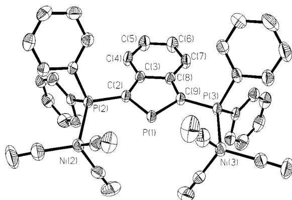
Figure 1. Representation of one of the two crystallographically independent anions in crystalline 4 [Li(THF) 4 ] (50% thermal ellipsoids); selected bond lengths [Å] and angles [°] (data of the second anion in brackets): P(1)–C(2) 1.732(4) [1.747(4)], P(1)–C(9) 1.736(4) [1.744(4)], C(2)–C(3) 1.441(5) [1.423(5)], C(2)–P(2) 1.789(4) [1.777(4)], C(3)–C(4) 1.416(5) [1.416(5)], C(3)–C(8) 1.432(5) [1.440(5)], C(4)–C(5) 1.367(5) [1.371(5)], C(5)–C(6) 1.399(6) [1.401(5)], C(6)–C(7) 1.372(5) [1.380(5)], C(7)–C(8) 1.413(5) [1.400(5)], C(8)–C(9) 1.440(5) [1.431(5)], C(9)–P(3) 1.780(4) [1.774(4)], P(2)–Ni(2) 2.241(1) [2.238(1)], P(3)–Ni(3) 2.241(1) [2.240(1)]; C(2)–P(1)–C(9) 93.0(2) [92.6(2)]
